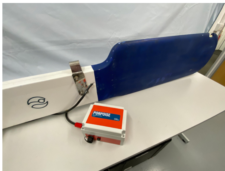
Image of the RS Aqua Porpoise hydrophone integrated with the rudder of a GB Row Challenge boat.
