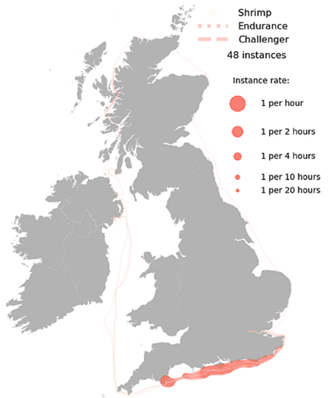
The underwater sound of snapping shrimp
